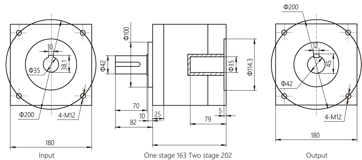
DIMENSION (mm)
