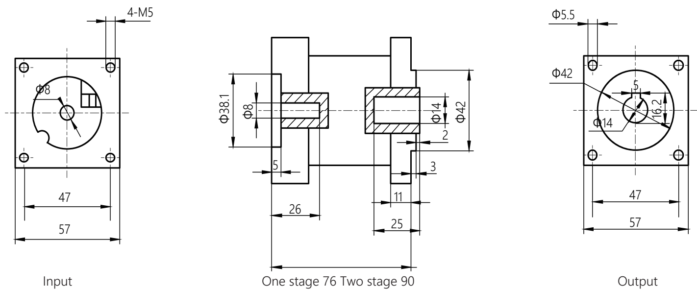
DIMENSION (mm)
