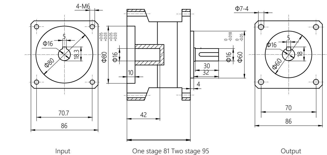
DIMENSION (mm)
