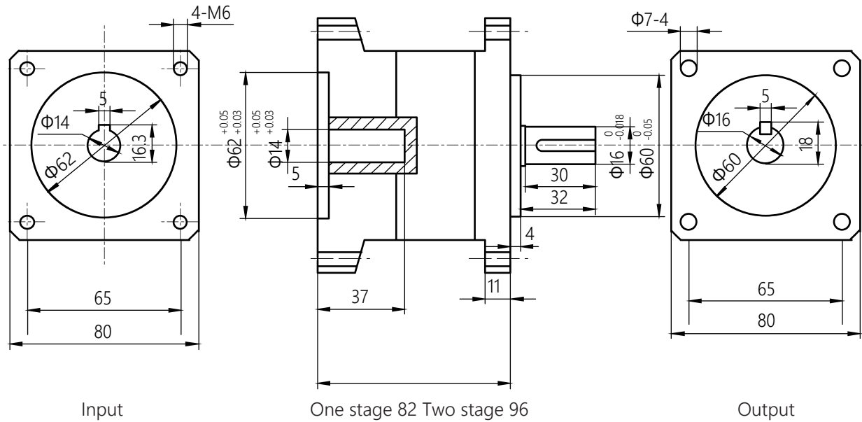
DIMENSION (mm)
