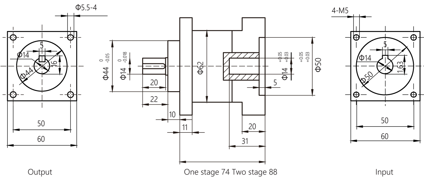
DIMENSION (mm)
