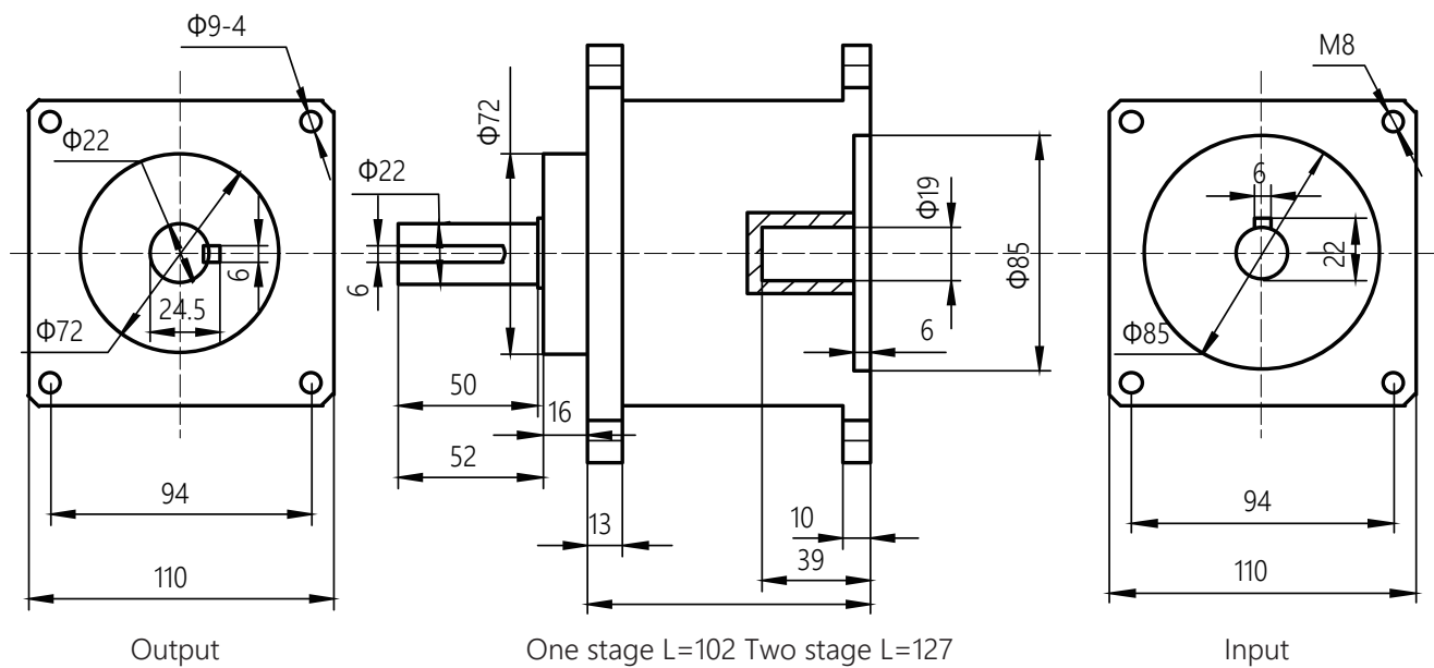
DIMENSION (mm)
