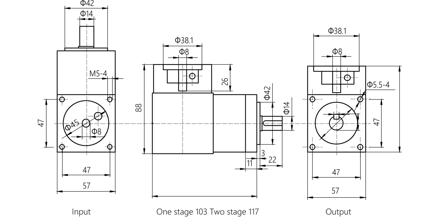
DIMENSION (mm)
