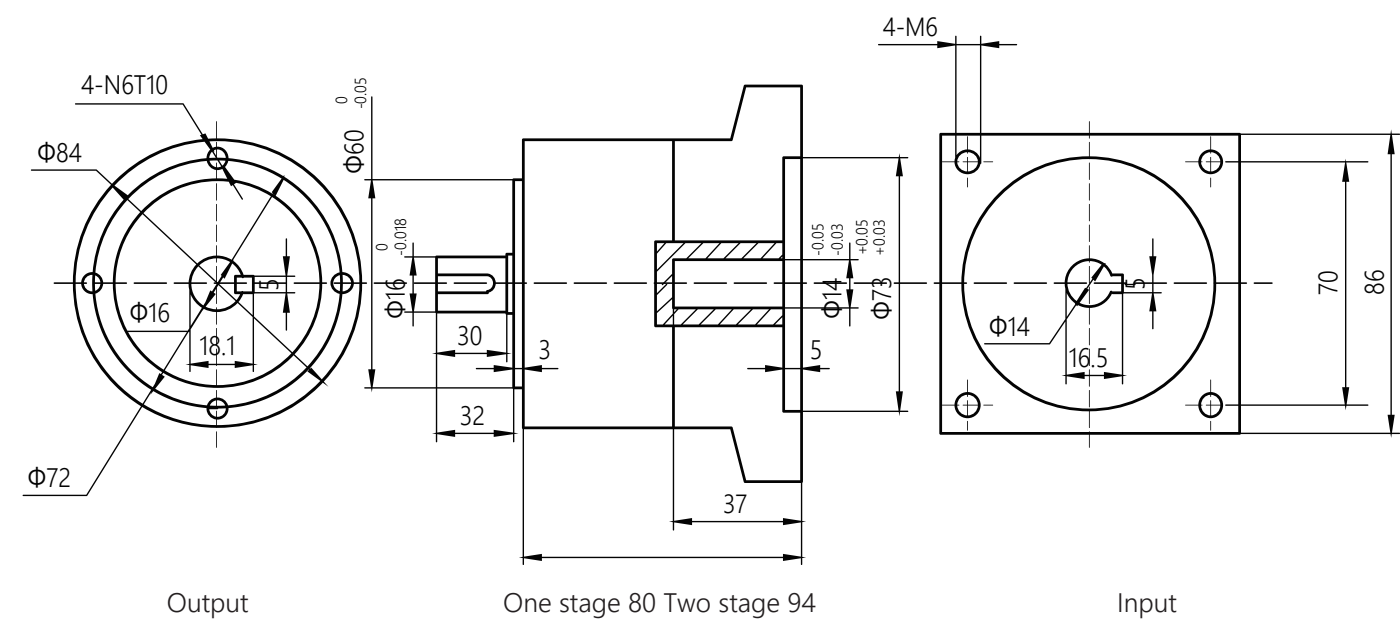
DIMENSION (mm)
