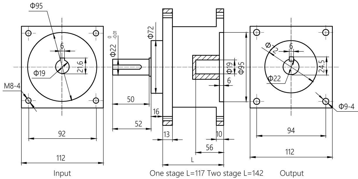
DIMENSION (mm)
