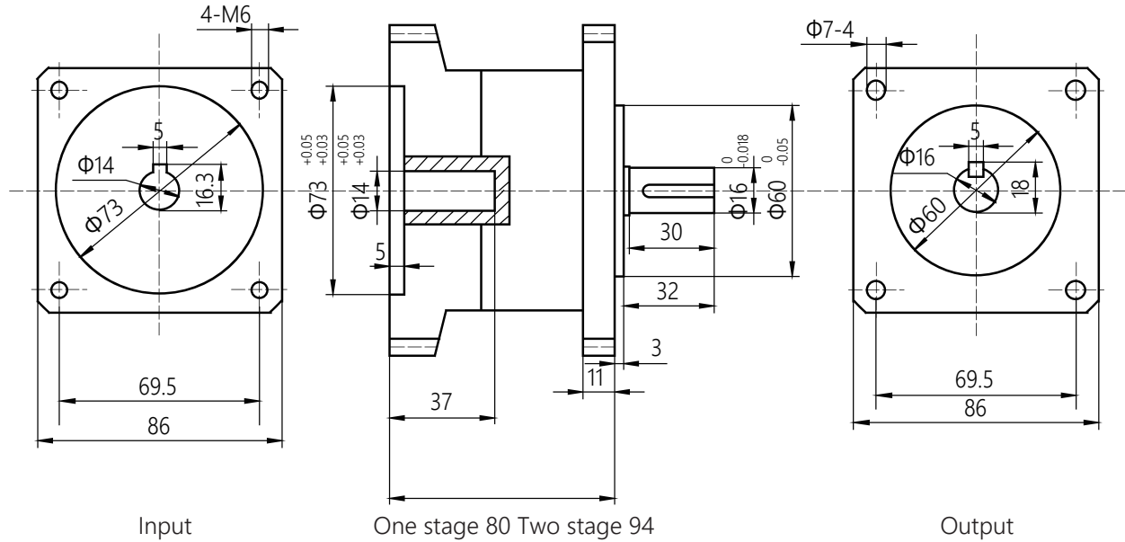
DIMENSION (mm)
