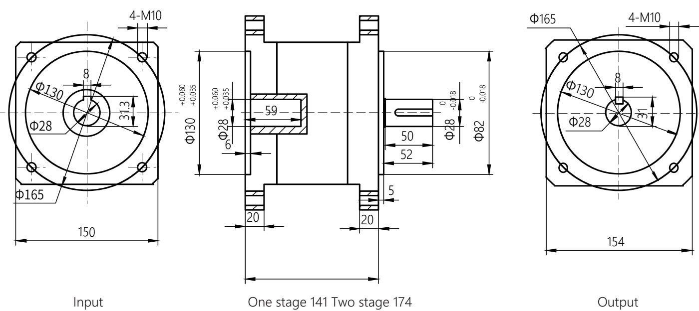
DIMENSION (mm)
