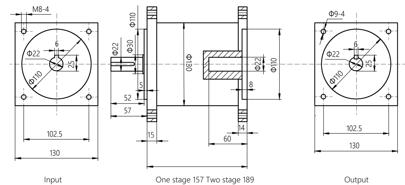
DIMENSION (mm)
