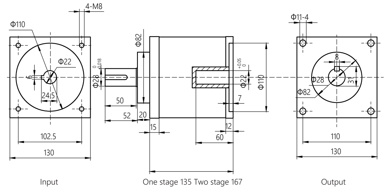
DIMENSION (mm)
