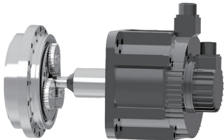
RV-SZ: Compact Design, Facilitates Sealing
