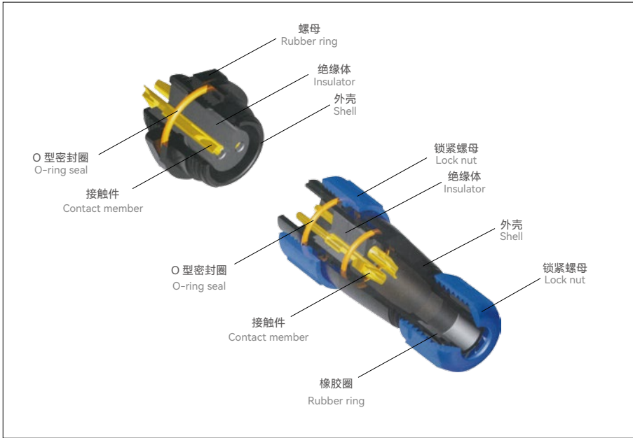
产品结构图 Product structure drawing
