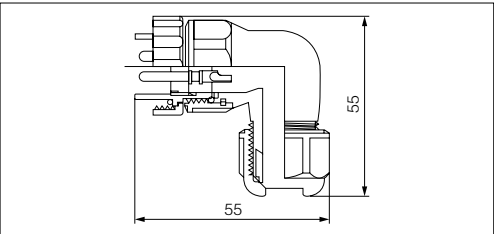
弯式带电缆锁紧插头 Bent plug with cable locking
