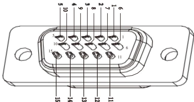
2.3.4 Communication signal connection (CN3) terminal definitions
